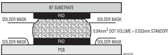
Figure A2. Good Mounting Depends on Standoff and Bump Volume
