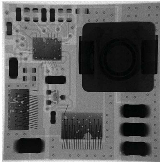
Figure 6. \mu Module X-ray Following a Correct Reflow and Rework Procedure
